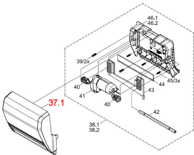
Figure 3 - T200-IDENT-PRINTER CUTTER/PERFORATOR
