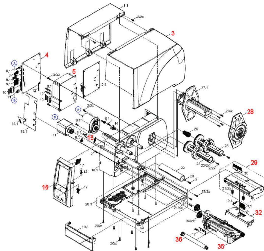
Figure 2 - T200-IDENT-PRINTER
