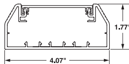
T-70 Internal Area = 5.15 Sq. In.
