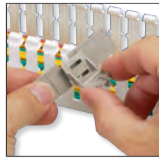
Labeling Outside Duct – Break off the last segment from wire retainer below 1.5" mark and snap onto the back of the remaining segment. Install label and mount between fingers facing outward.
